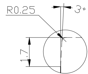
Detail Q
